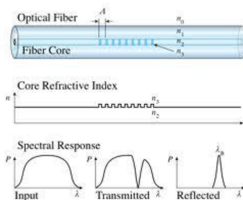
Fibre Bragg Grating: Light with a wavelength matching the gratings resonant wavelength experiences strong reflection back along the fibre. This resonant wavelength is strain/temperature dependent which provides the basis of strain and temperature sensing using the device.
